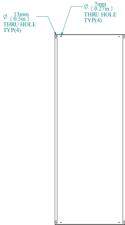
REAR VIEW
