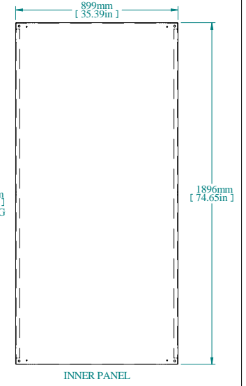
INNER PANEL
