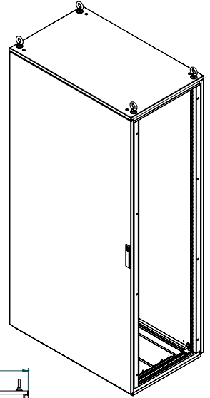
ISOMETRIC VIEW
