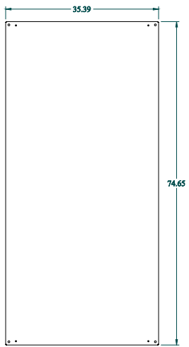
INNER PANEL
