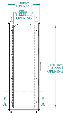
L.S. VIEW
