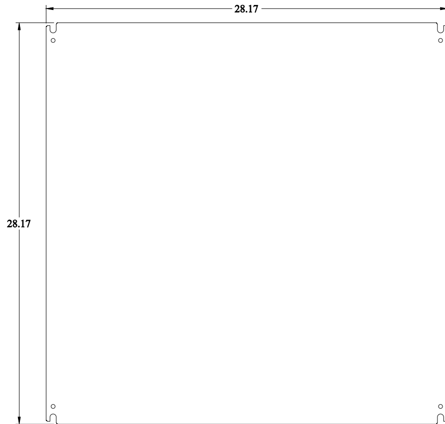
FRONT VIEW
