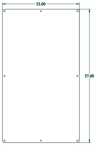
INNER PANEL
