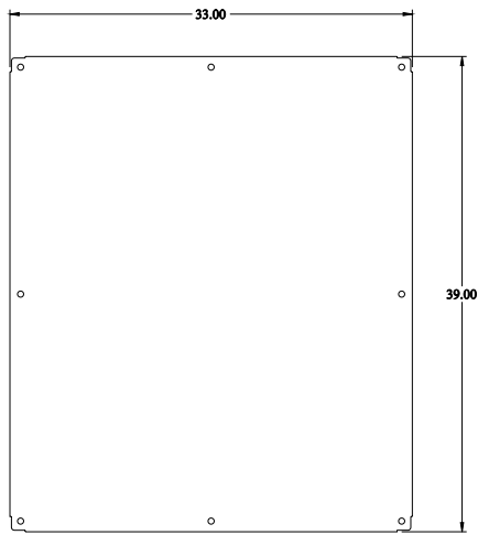
INNER PANEL
