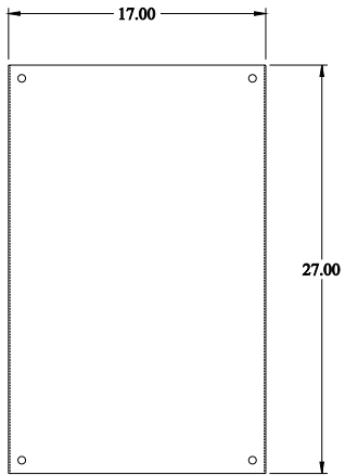
INNER PANEL
