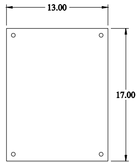
INNER PANEL
