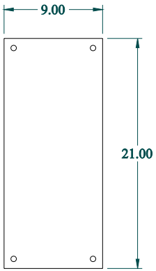
INNER PANEL
