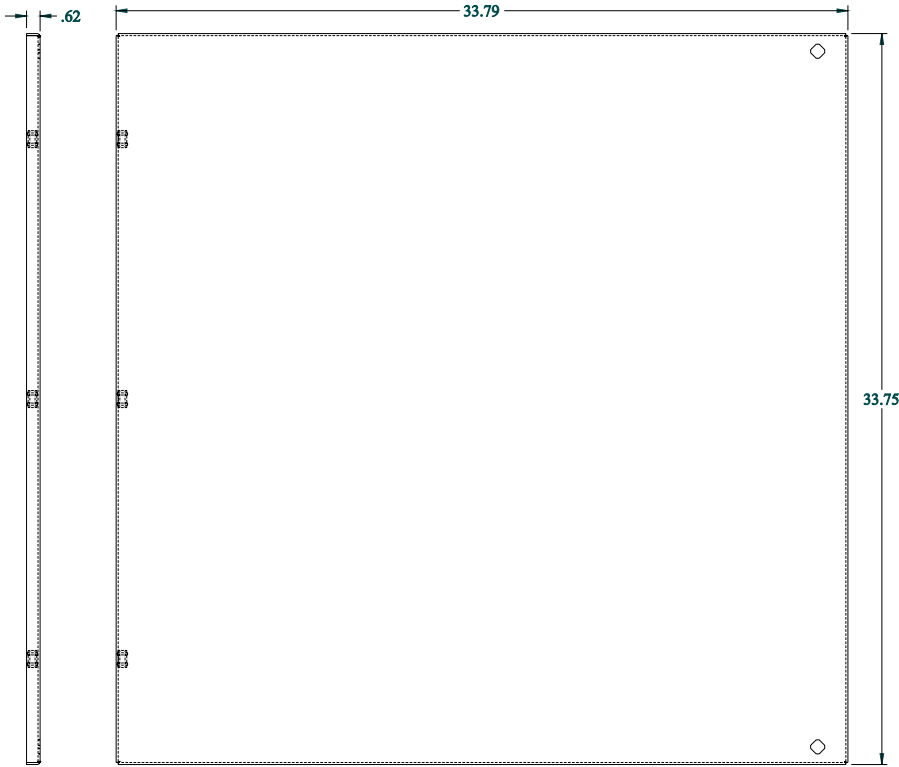
SIDE VIEW
