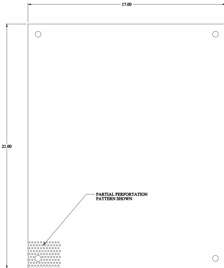
FRONT VIEW
