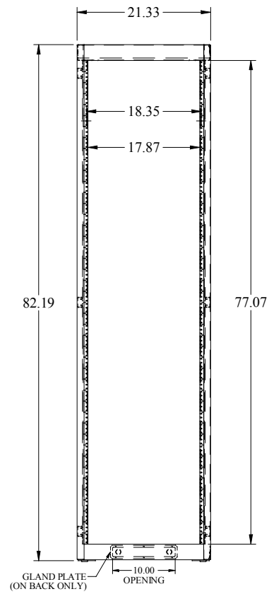
FRONT VIEW
