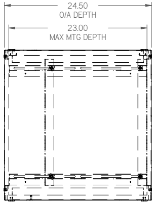
L.S. VIEW
