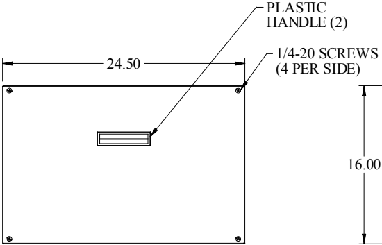
L.S. VIEW
