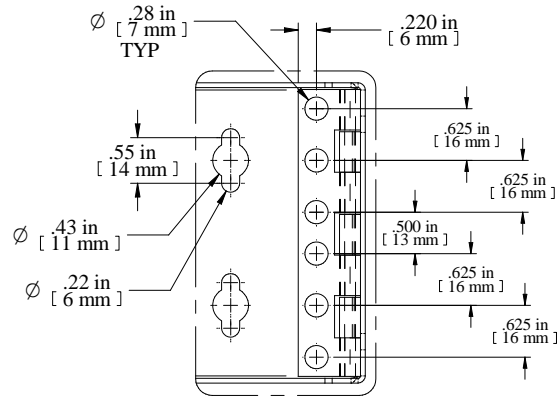
DETAIL A 3:1
