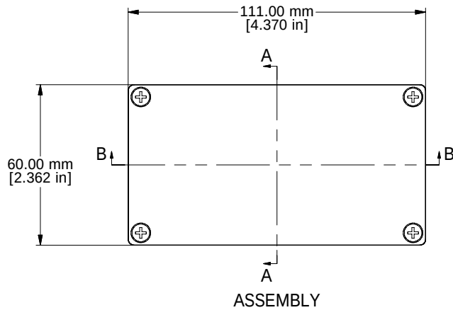
ASSEMBLY
