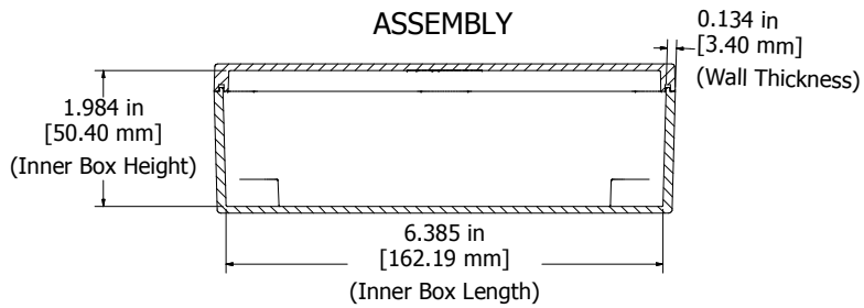
SECTION N-N Side View of Assembly
