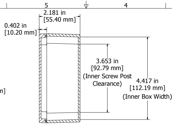
SECTION R-R End View of Assembly
