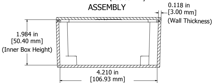
SECTION L-L Side View of Assembly
