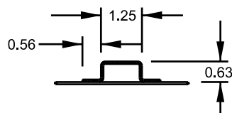
Section Z-Z
