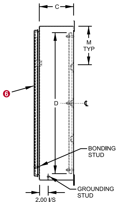
Formed View
