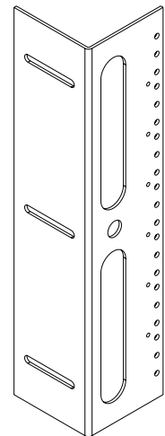
ISOMETRIC VIEW
