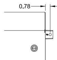
Mounting Foot Detail
