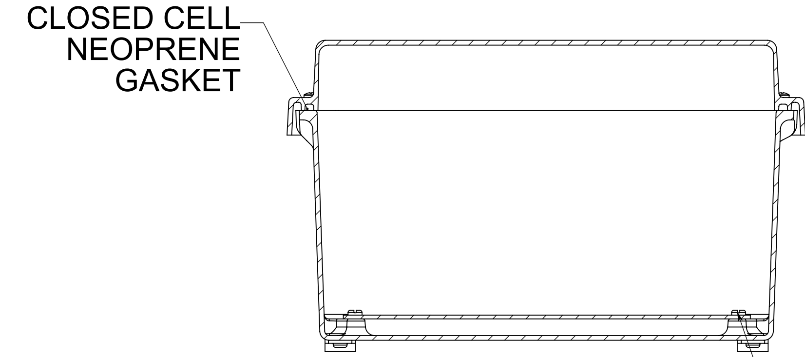
SECTION B-B
