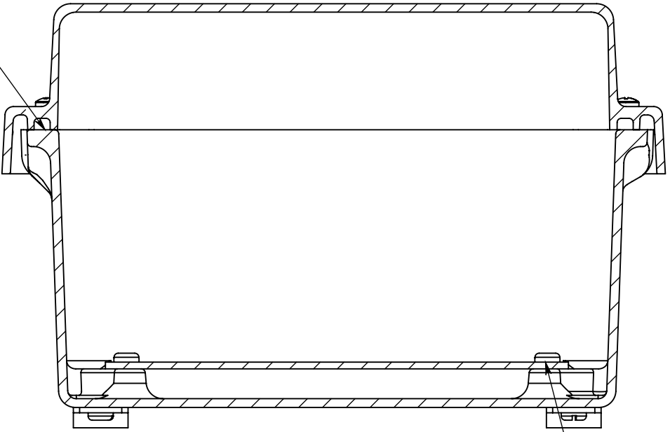
SECTION B-B
