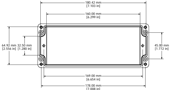
BOX - INSIDE
