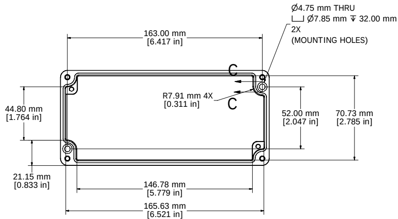
BOX - INSIDE
