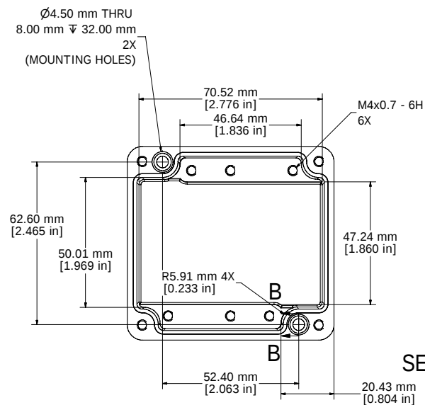
BOX - INSIDE
