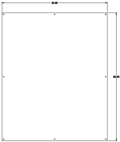
INNER PANEL
