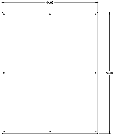
INNER PANEL
