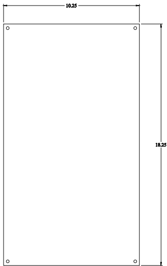
INNER PANEL
