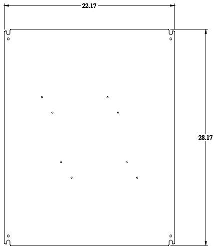
INNER PANEL
