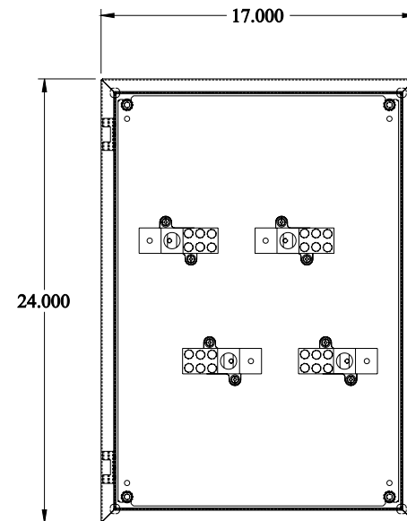
FRONT VIEW - COVER REMOVED
