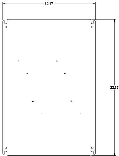
INNER PANEL
