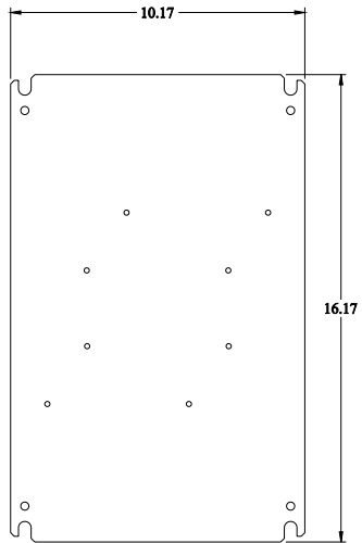
INNER PANEL
