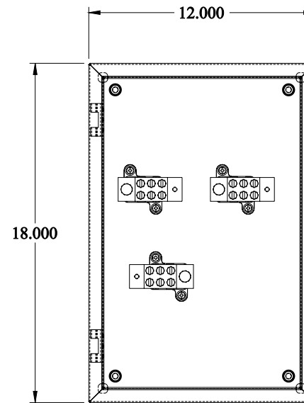
FRONT VIEW - COVER REMOVED
