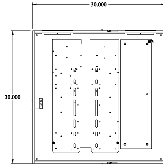
FRONT VIEW - DOORS REMOVED
