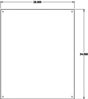
INNER PANEL
