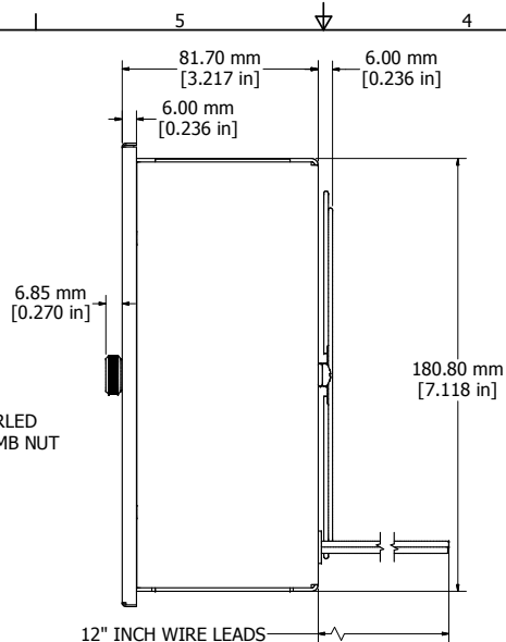
ASSEMBLY - VIEW FROM SIDE
