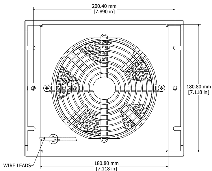
ASSEMBLY - VIEW FROM BACK
